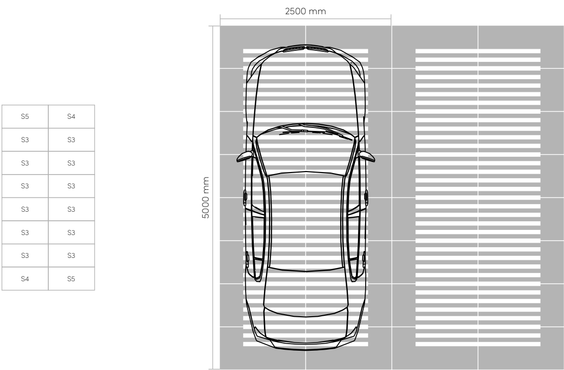
COMBINATION OF TILES S3, S4 & S5
