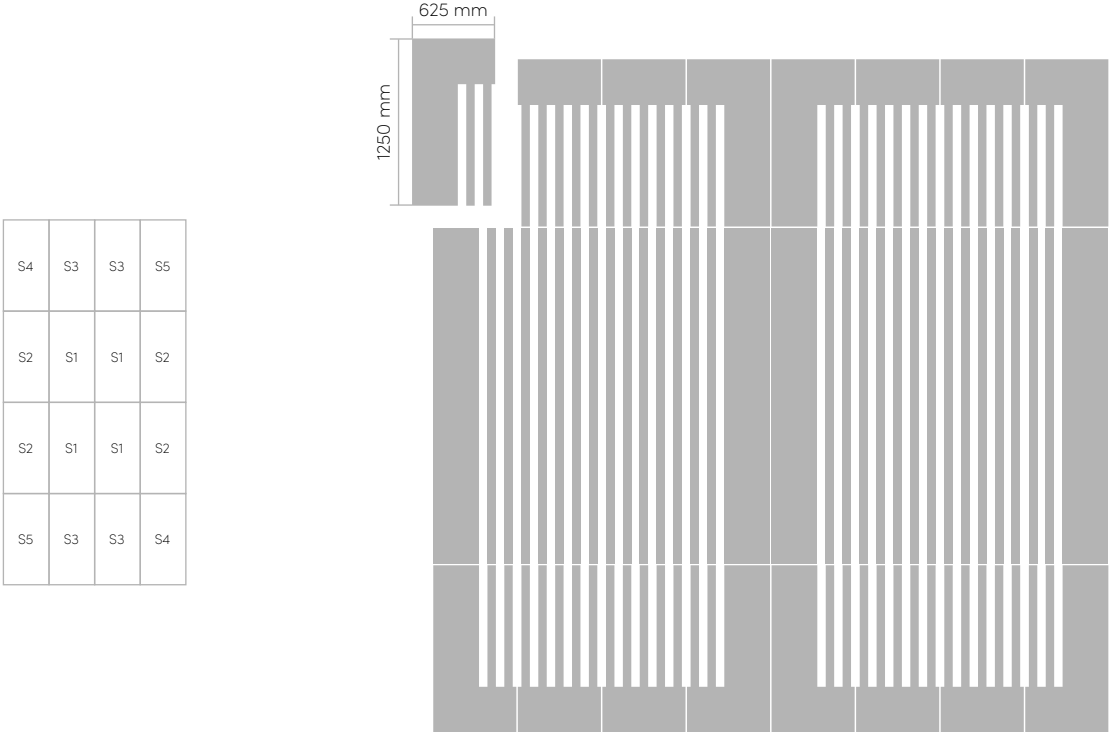
COMBINATION OF TILES S1, S2, S3, S4 & S5
