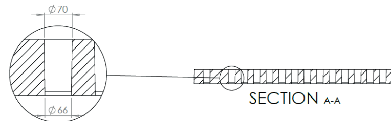
DETAIL G SCALE 1 : 5
